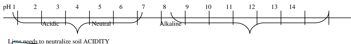
Fig. 1. pH Scale Chart (after Stamp, Martin and Leonard, 1976)
