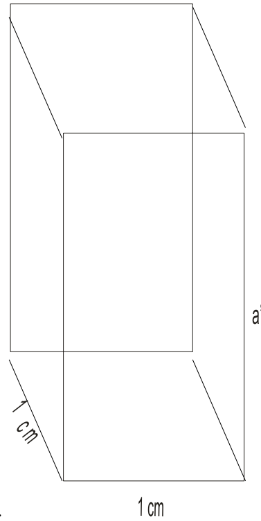
Fig. 1.1: Illustration of a 'cm of rainfall (after Ogunrinde, Sam.I; 1996)
