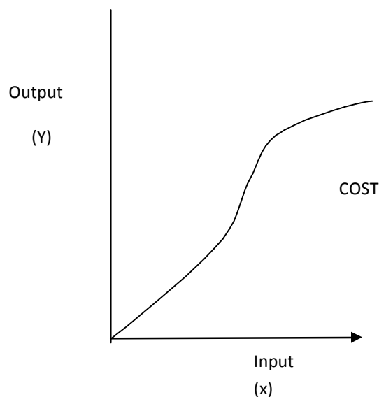
Fig. 19: Production Function
