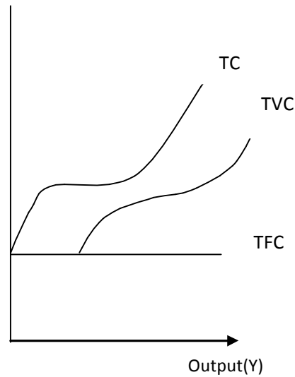
Fig. 20: Cost Functions
