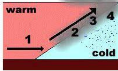
Fig. 8: Frontal rainfall
