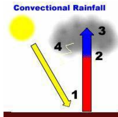
Fig. 6: Convictional rainfall
