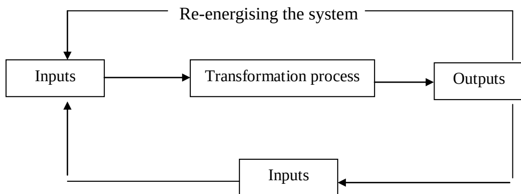
Fig. 1.3: Input-Output Model
