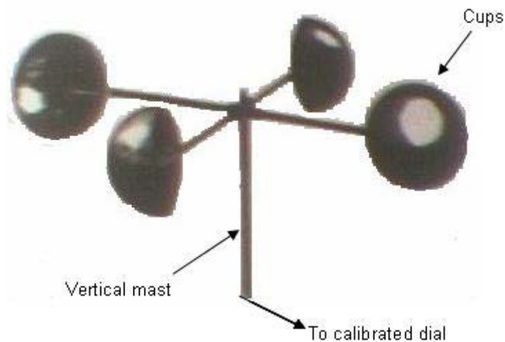
Fig. 19: Wind aneometer
