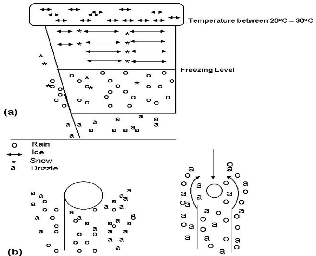
Fig. 5: Processes of raindrop formation according to (a) Bergeron-Findeisen theory and (b) coalescence theory (Source: Ayode, 2004)
