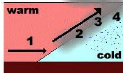
Fig. 8: Frontal rainfall
