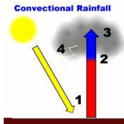
Fig. 6: Convictional rainfall
