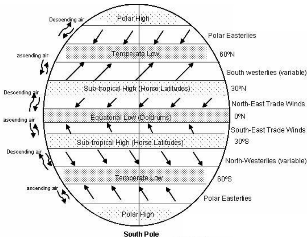
Fig. 4: World pressure belts and planetary winds
