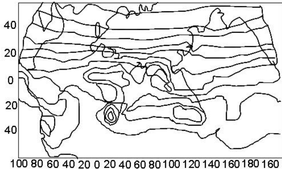
Fig. 9(a): Global distribution of insolation in December in kcal/cm 2 per month, (Source: Ayoade, 2002)
