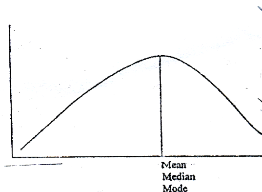
Fig. 6: Normal Distribution
