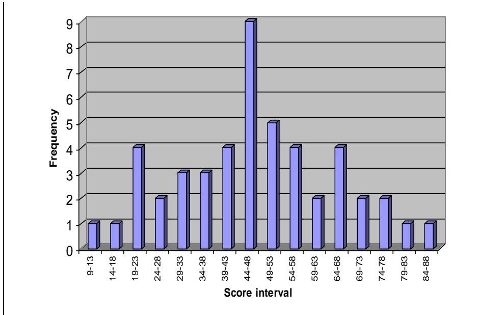
Fig. 1: Frequency Distribution
