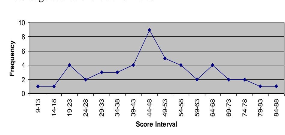
Fig. 2: Frequency Polygon
