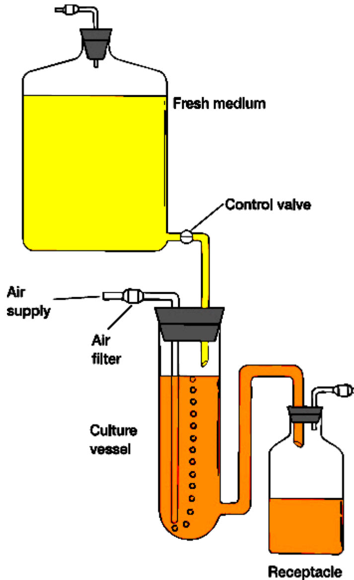
Fig.1.3: A Continuous Culture Systems: The Chemostat
