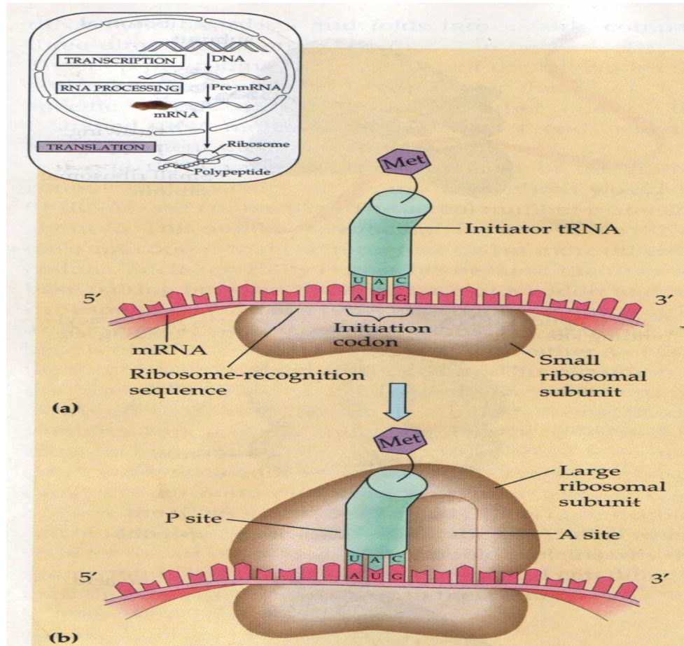
Figure 4. Chain Initiation
