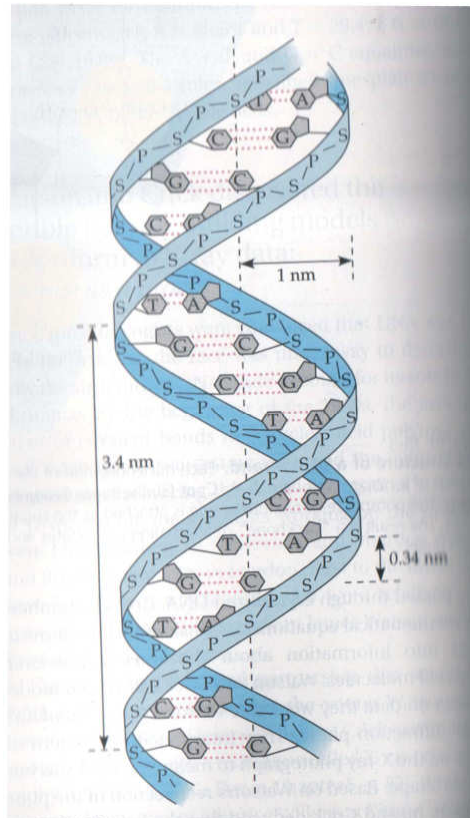
Figure 2. DNA Structure
