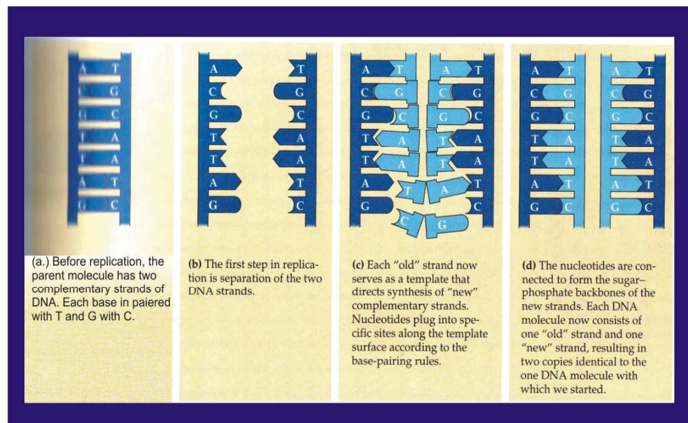
Figure 3. DNA Replication
