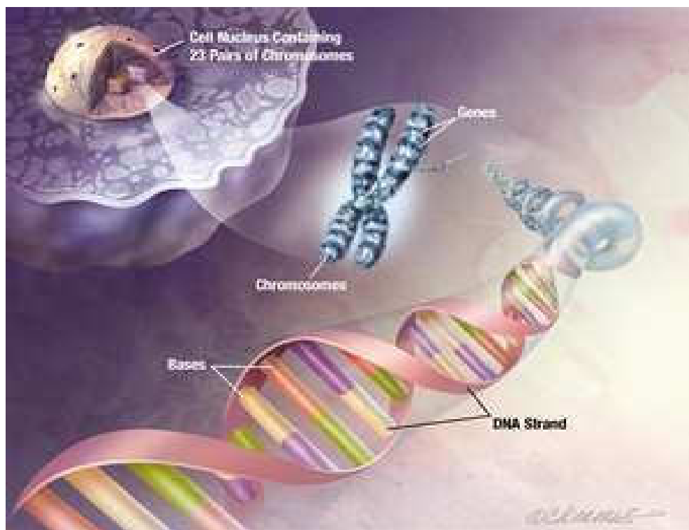
Figure 1. Chromosome structure
