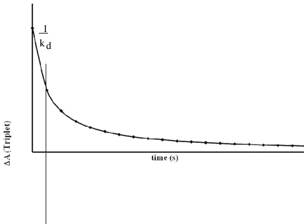
Figure X: A typical triplet absorption curve (simulated)
