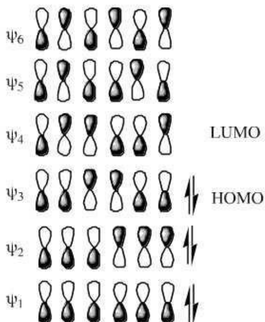
Figure 7: Superimposition of HOMO upon triene system
