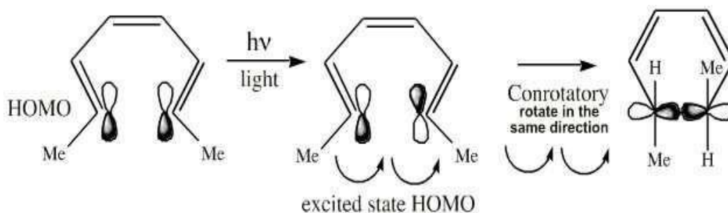
Figure 9: Conrotation of photoexcited System
