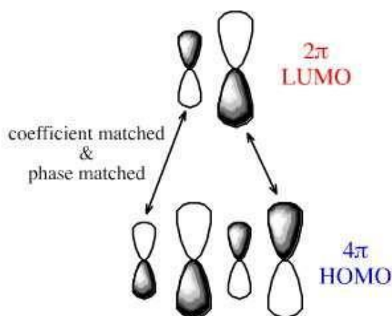
Figure 6: Coefficient and phase matched HOMO/LUMO
