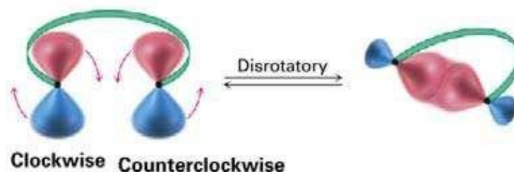
Figure 2: Conrotatory and Disrotatory twisting
