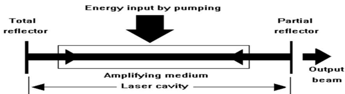
Figure 12: Light amplification in the LASER cavity
