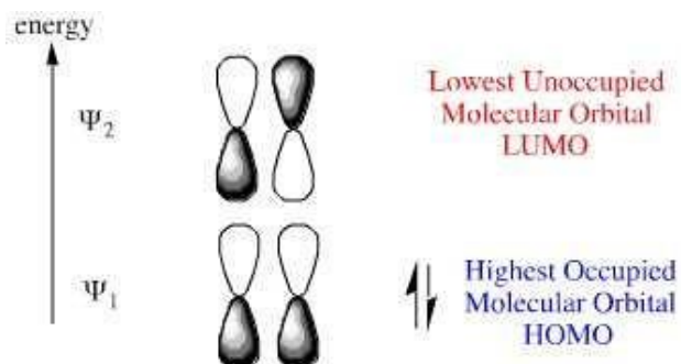
Figure 3: HOMO/LUMO components of a dienophile
