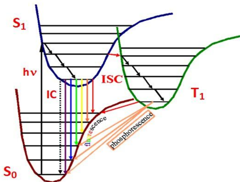
Figure 3: The photophysical processes fluorescence, vibrational relaxation, internal conversion, intersystem crossing, and phosphorescence.
