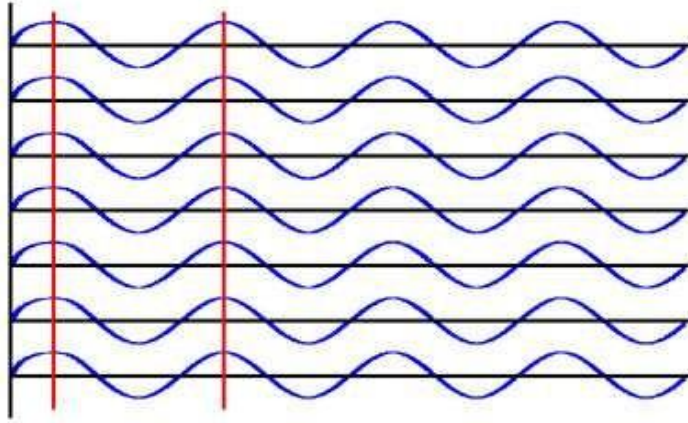
Figure 6: Coherent light waves
