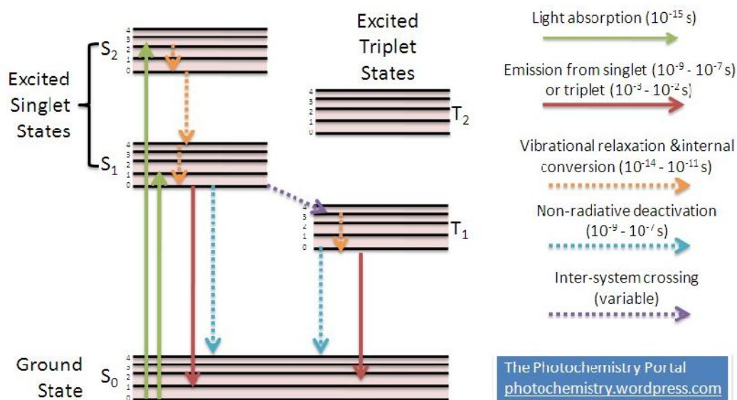
Figure 4: A Jablonski diagram for an organic molecule.
