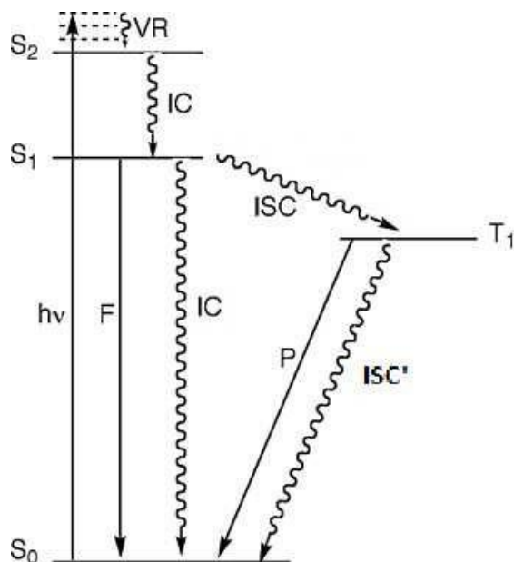
Figure X: Jablonski diagram showing processes at the S 1 and T 1 states
