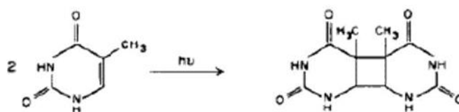
THYMININE DIMER
