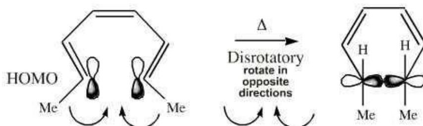
Figure 8: Disrotatory twist of HOMO
