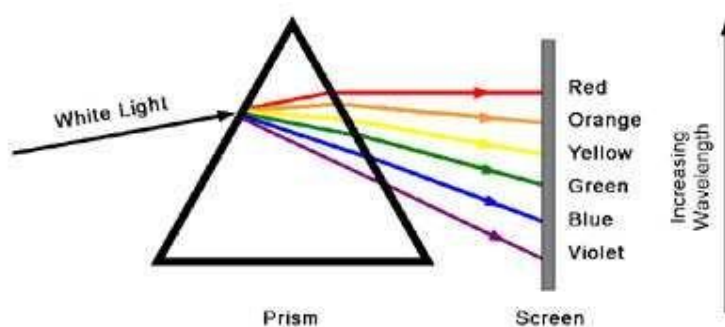
Figure 2: Dispersion of white light by a prism
