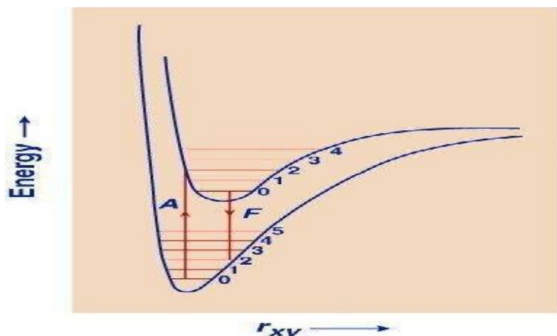
Figure 5: Frank-Condon Principle. Potential energy curves for the ground state and an excited state of a diatomic molecule. ( r , interatomic distance; A , absorption; F , fluorescence; numbers indicate vibrational states).
