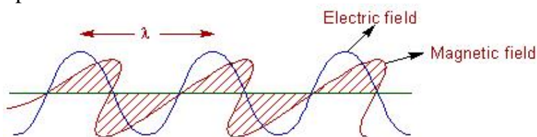
Figure 2: Electromagnetic Radiation
