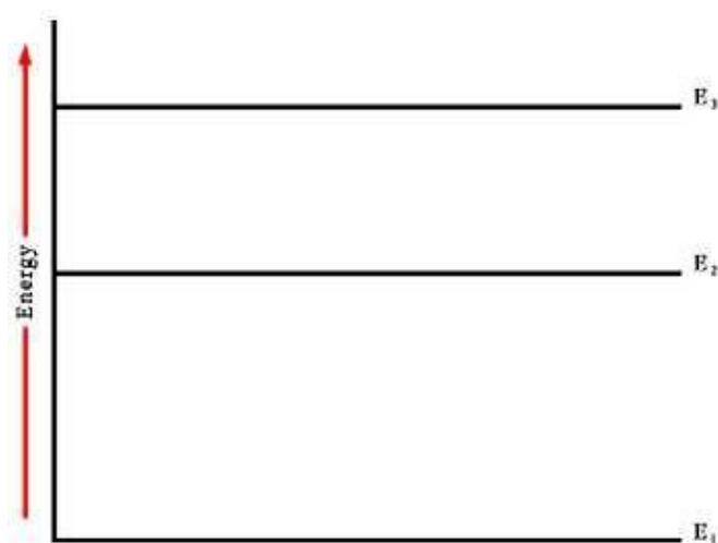
Figure 8: Atomic energy-level diagram
