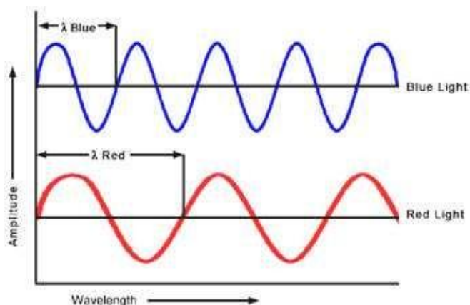
Figure 1: Comparison of the wavelengths of red and blue light
