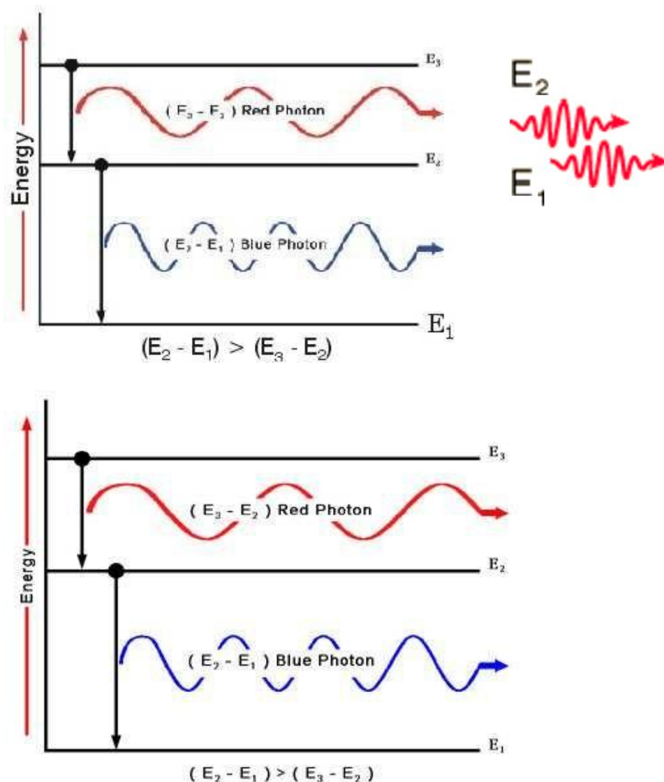
Figure 9: Spontaneous emission
