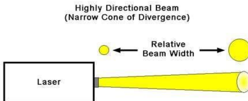
Figure 4: Directionality of laser light
