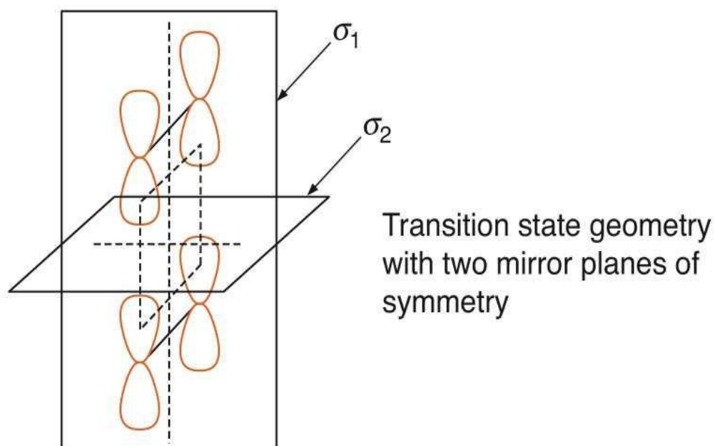
Figure 1: Transition state geometry with two mirror planes of symmetry
