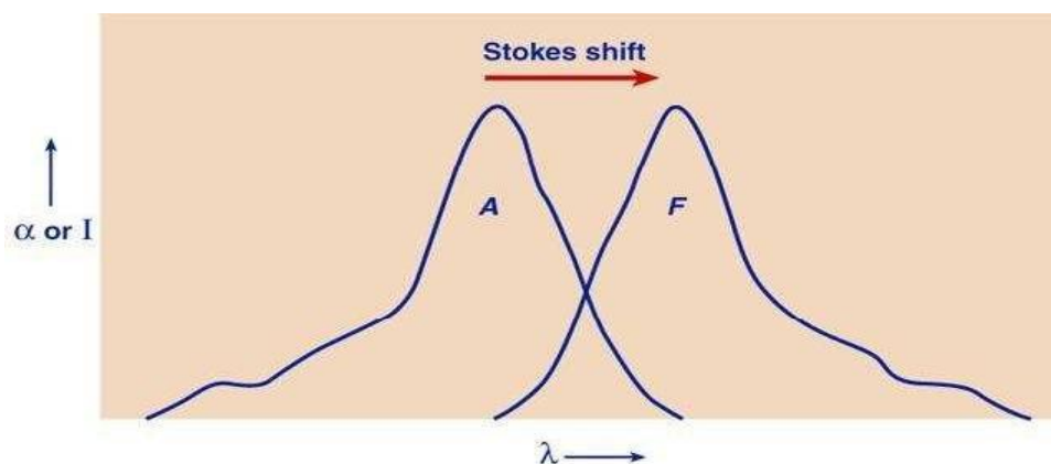
Figure 6: The Stokes' shift (displacement of fluorescence band compared to the absorption band of a molecule). Approximate mirror symmetry of the two bands exists when the shapes of the potential curves in the ground state and the excited state are similar.
