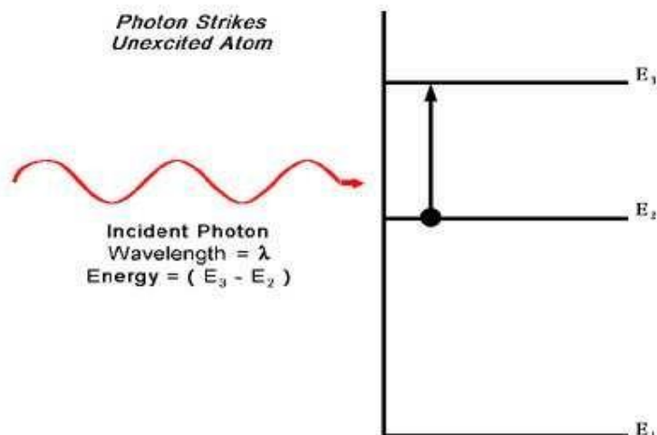
Figure 11: Absorption of light
