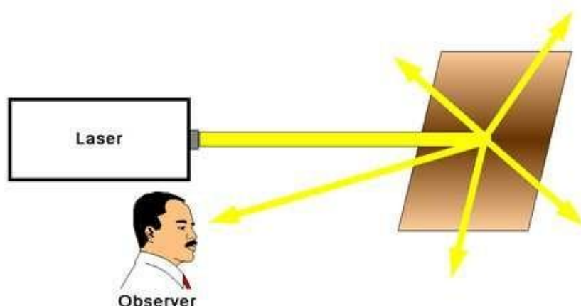
Figure 7: The beam of a low-powered laser strikes a rough surface
