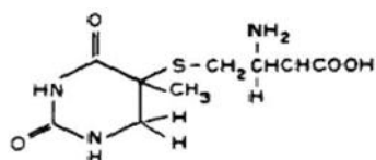
5-S-CYSTEINYL-6-HYDROTHYMININE
