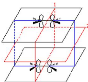
Figure 2: Two ethylene molecules going Head-to-Head
