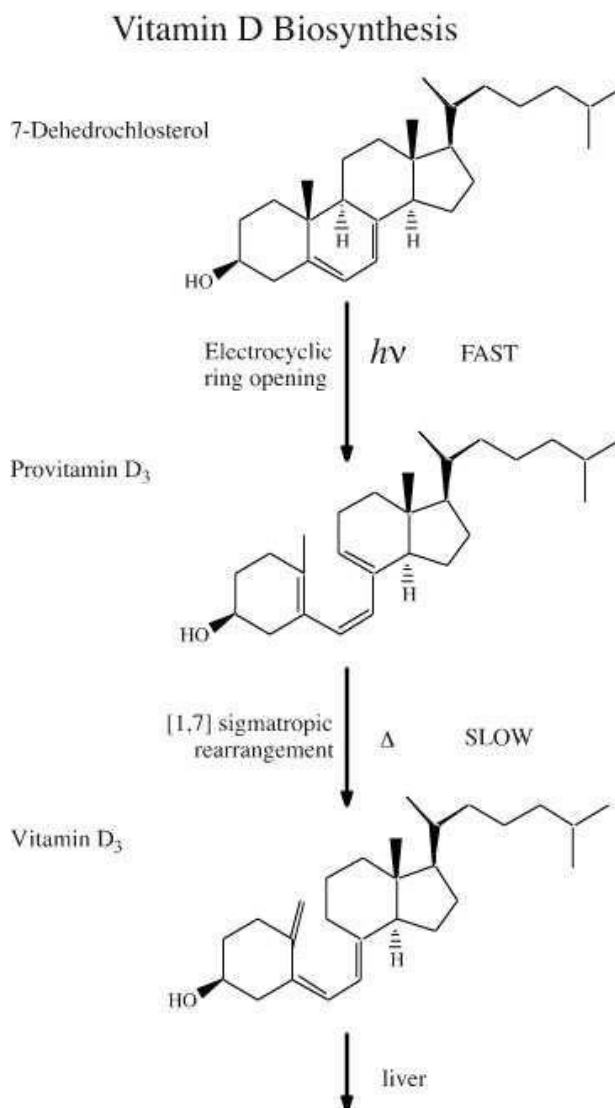
Figure 1 Sigmatropic rearrangement in biosynthesis of vitamin D
