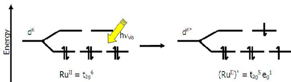
Figure 2: Absorption of a photon of visible light causes a d-d transition in Ru(II) giving the molecule a visible colour.
