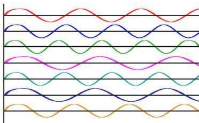
Figure 5: Incoherent light waves
