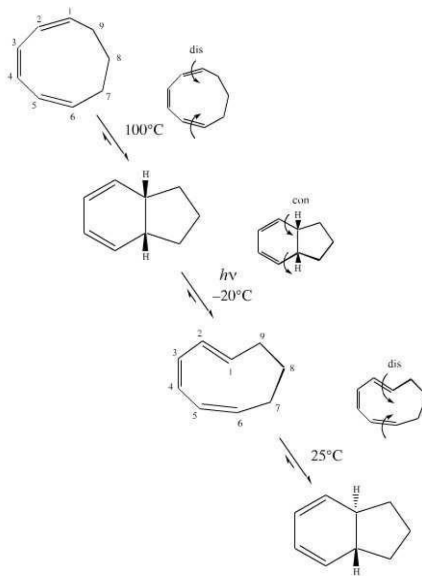
Figure 10 Conrotatory twist of 1,3,5-cyclononatriene
