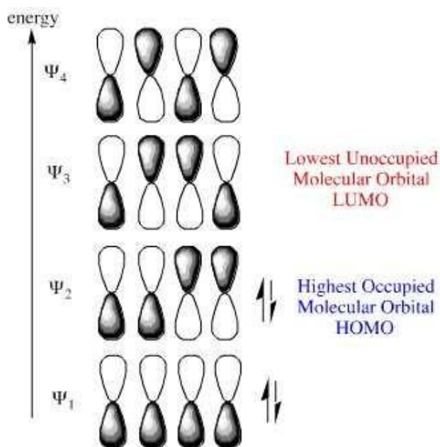
Figure 4: HOMO/LUMO components of a diene
