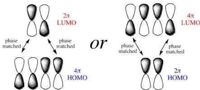
Figure 5: LUMO/HOMO interactions of diene and dienophile
