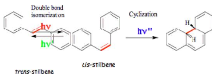
Scheme 1: Photochemical transformation of stilbene
