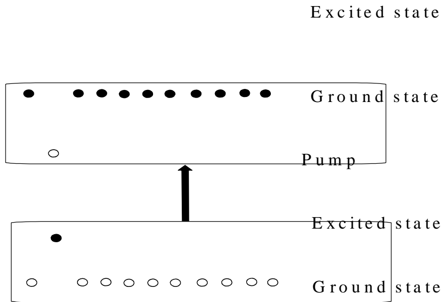
Figure 15: Population inversion in LASER systems
