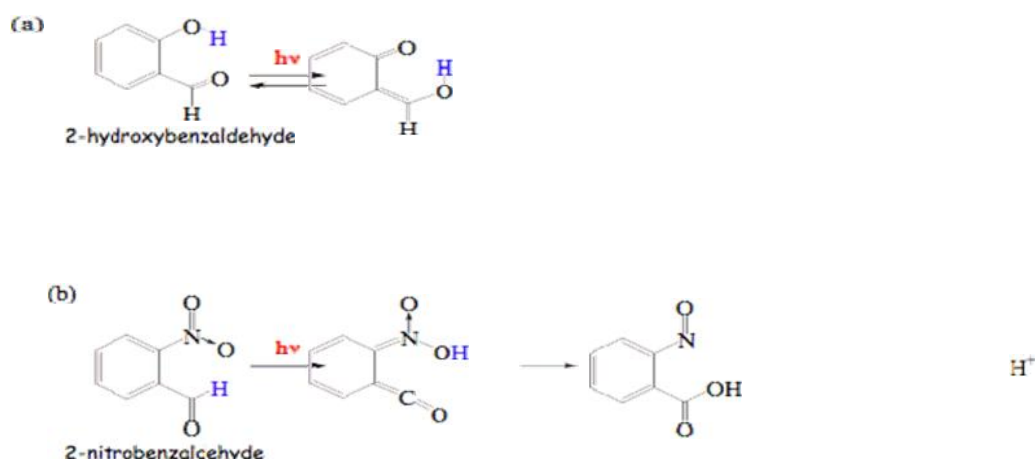
Scheme 2: Photochemical transformation of 2-nitrobenzaldehyde
