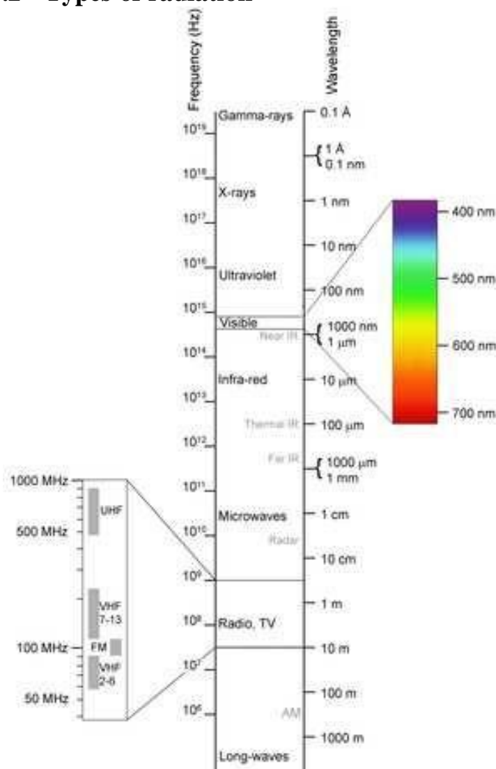
Figure 1: The electromagnetic spectrum
