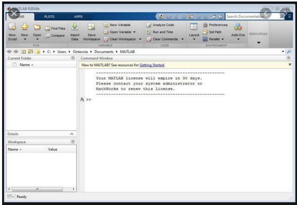
Figure 2: MATLAB
