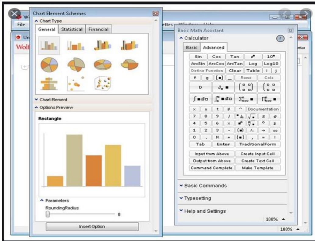
Figure 3: Mathemtica
