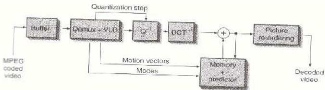
Figure 3.2.3b: Schematic diagram of the MPEG decoder
