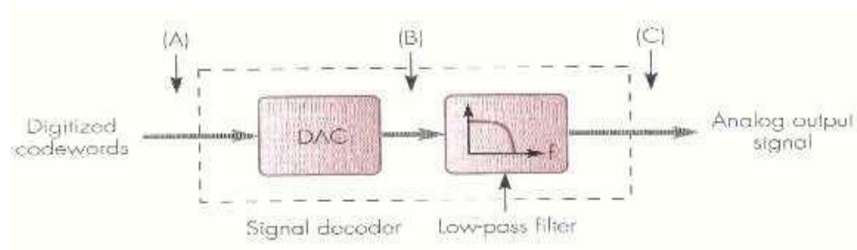
Figure 3.4.2 Source [Halsall, 2001]
