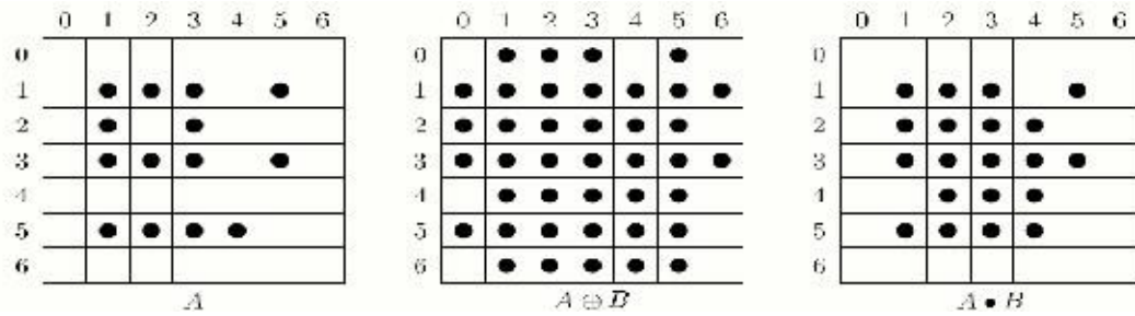
Figure 3.3b: Closing
