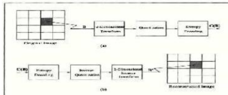
Figure 3.5.4: Transform Coding
