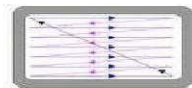
Figure 3.4: Raster Scan
