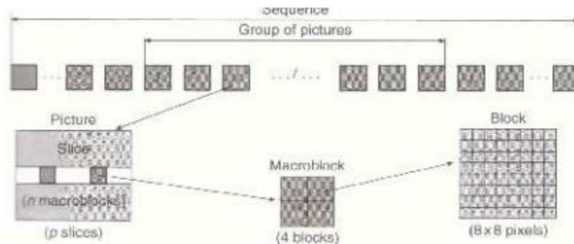
Figure 3.2.2a: Hierarchy of the MPEG VIDEO layer
