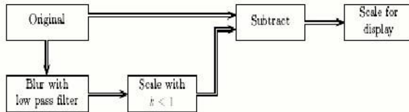
Figure 3.1.3a: Schema for Unsharp masking
