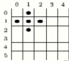
Figure 3.1.1a: Binary
