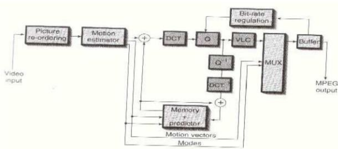
Figure 3.2.3a: Schematic diagram of the MPEG encoder
