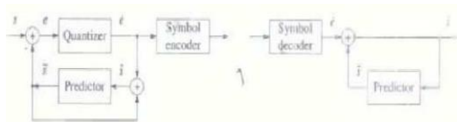
Figure 3.5.3: A predictive coding system
