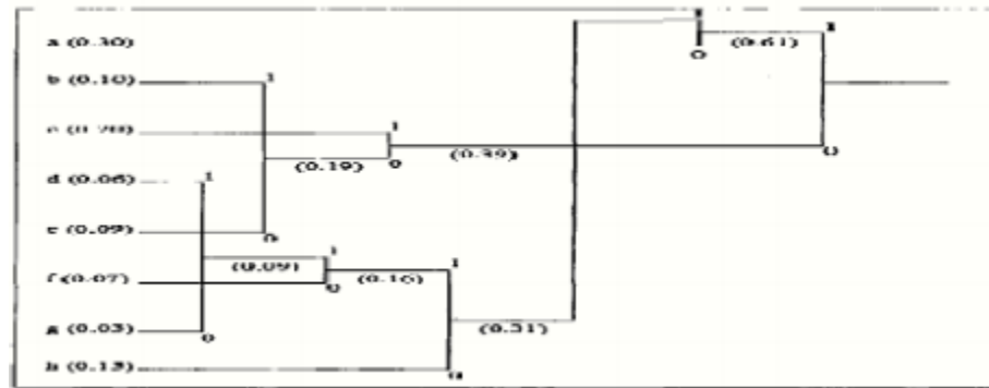
Figure 3.5.2: An example of Huffman Tree form by Applying Huffman algorithm Source [ Mitra and Tinkuachar, 2003]
