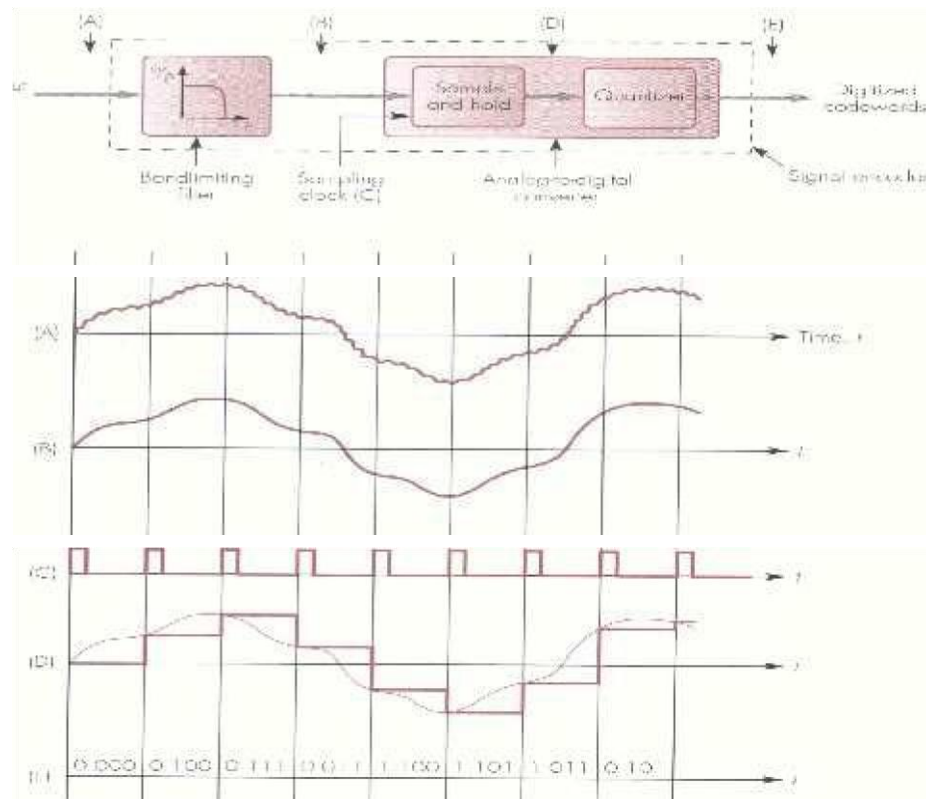
Figure 3.4.1: Analog to digital signal conversion Source [Halsall, 2001]
