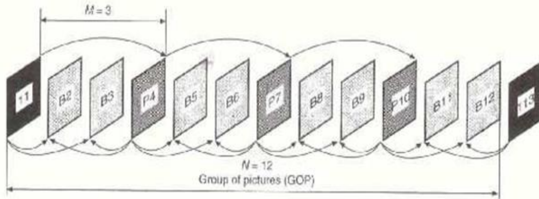
Figure 3.2.1b Example of an MPEG group of pictures for M=3 and N=12
