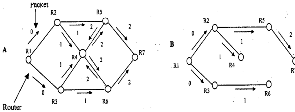
Figure 3.13(a): Flooding Figure 3.13(b): Spanning Tree
