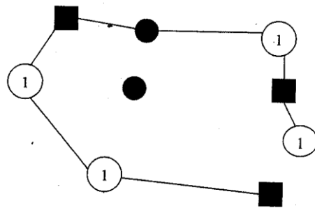
Figure 3.27: A pruned spanning multicast tree for group 1
