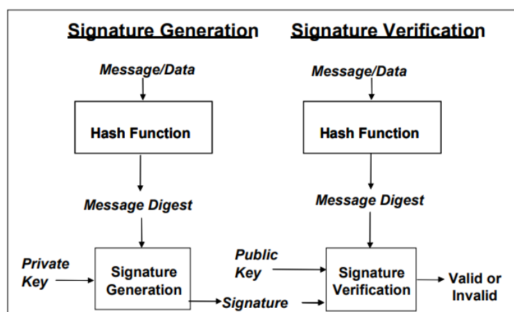
Figure 4.27: Digital signature verification process
