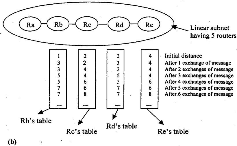
Figure 3.17 (b): Count to infinity problem
