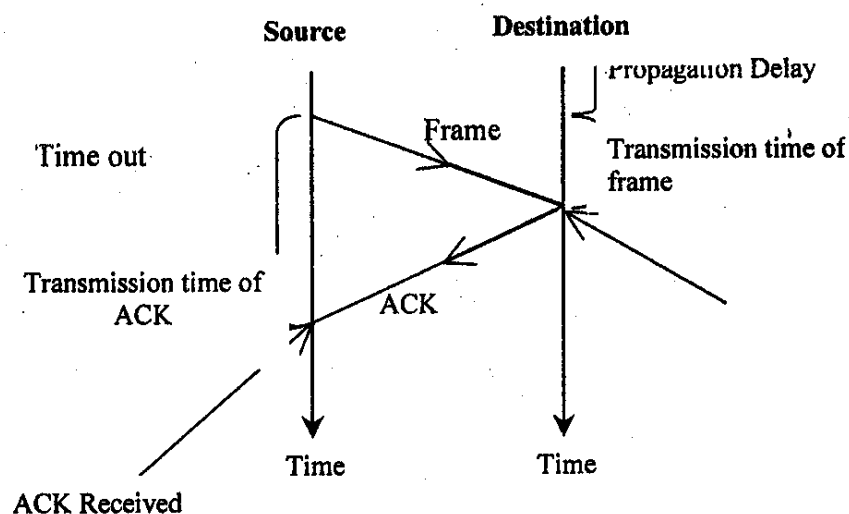
Figure 2.15: Stop and Wait
