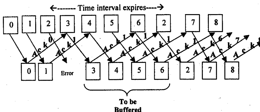
Figure 2.26: Selective Repeat
