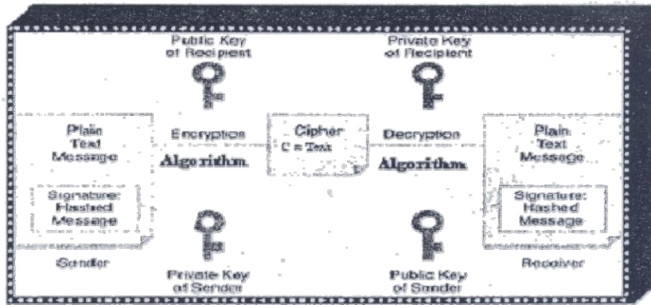
Figure 4.32: Encryption and signing using public key cryptography
