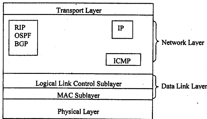
Figure 3.37: Network layer protocols
