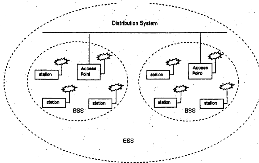
Figure 2.40: Wireless LAN architecture
