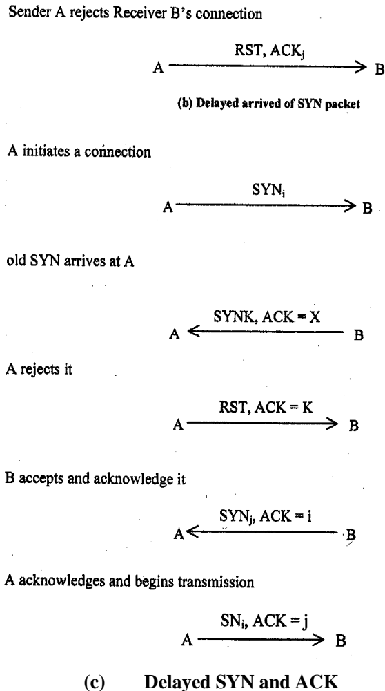
Figure 4.7: Three-way handshake mechanism
