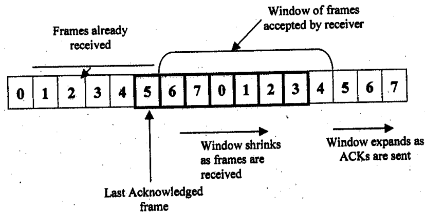
Figure 2.18: Receiving window in 1 sliding window
