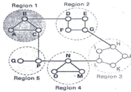
Figure 3.24: Hierarchical routing
