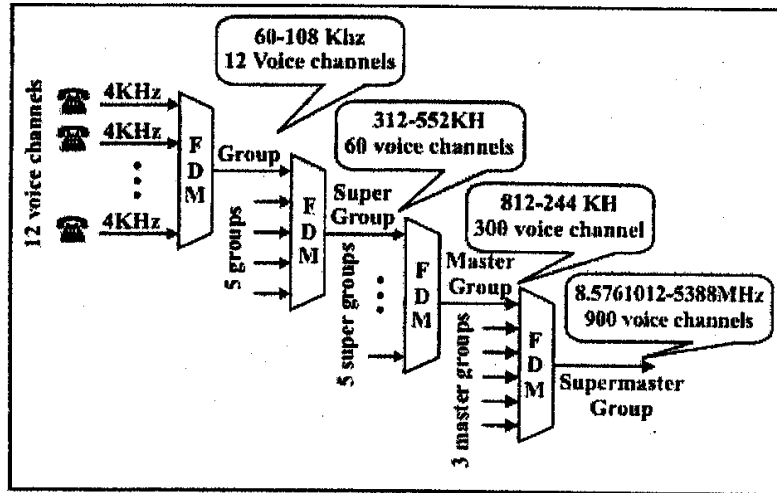
Figure 1.51: Analogue hierarchy
