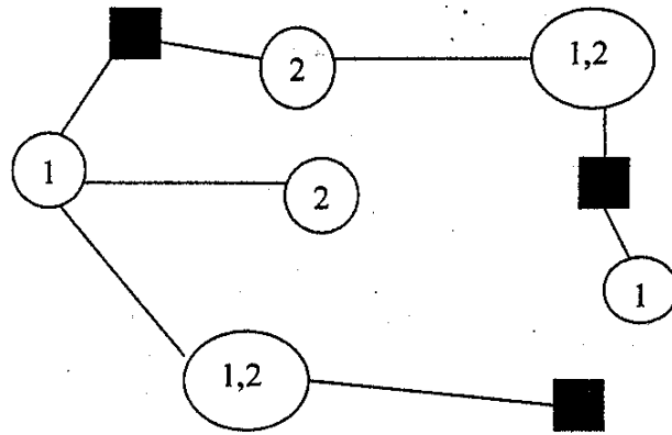
Figure 3.26: Spanning tree for the leftmost router
