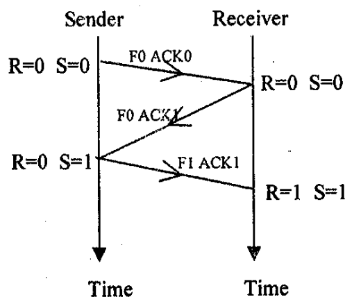
Figure 2. 24: Piggybacking 1
