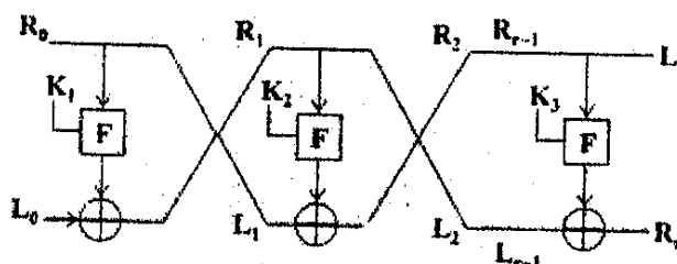
Figure 4.16: Feistel' Cipher
