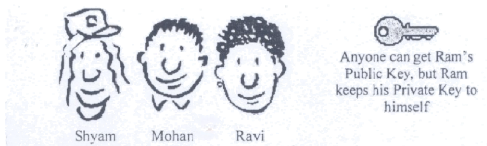
Figure 4.34: Ram's co-workers
