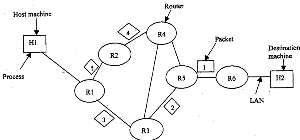
Figure 3.4: Routing in a datagram subnet
