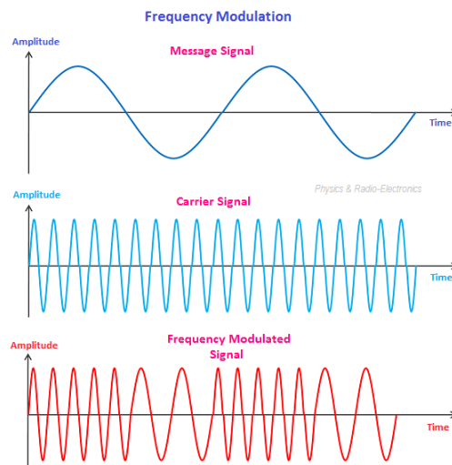
Figure 1.36: Frequency modulation
