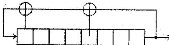
Figure 4.13: Stream cipher linear feedback shift register (LFSR)
