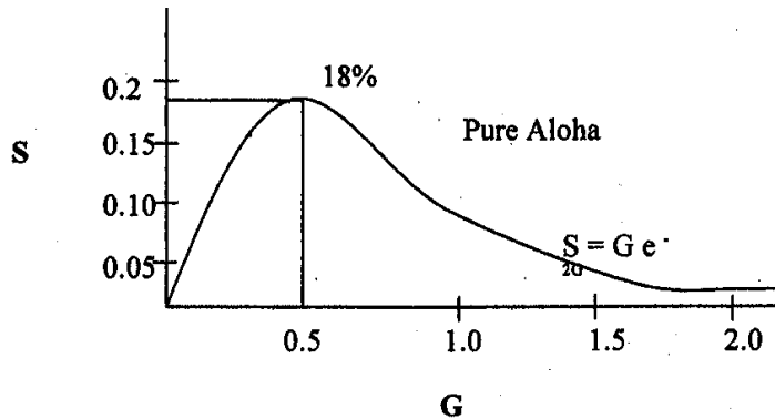
Figure 2.34: Throughput vs. load graph of pure ALOHA
