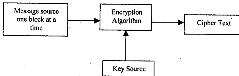
Figure 4.12: Block cipher
