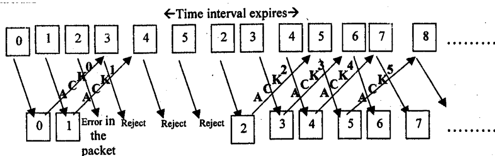
Figure 2. 25: Go-Back-N
