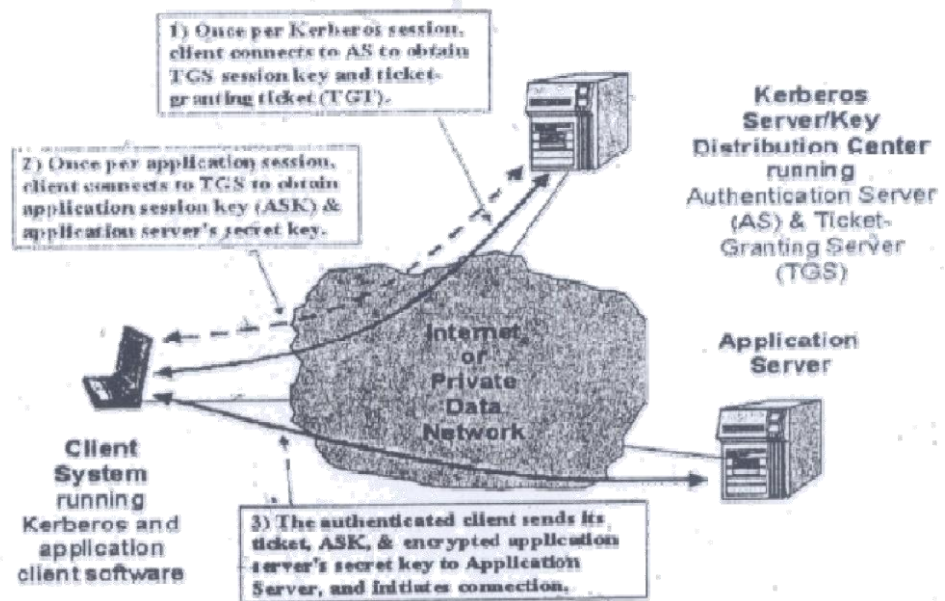
Figure 4.45: Kerberos
