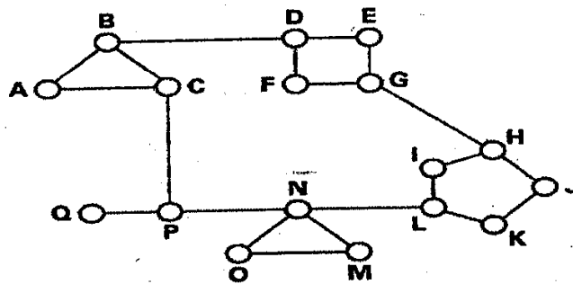
Figure 3.22: Network graph
