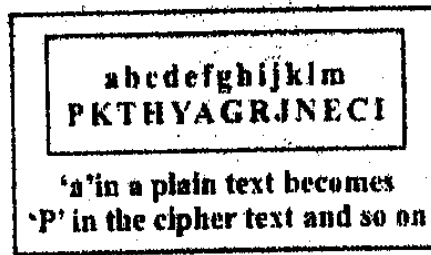
Figure 4.14: Substitution
