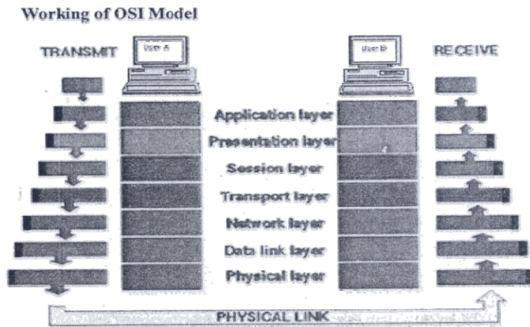
Figure 1.11: Working of OSI Reference Model
