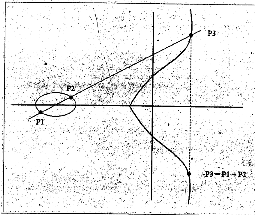
Figure 4.29: Elliptic Curve Cryptography
