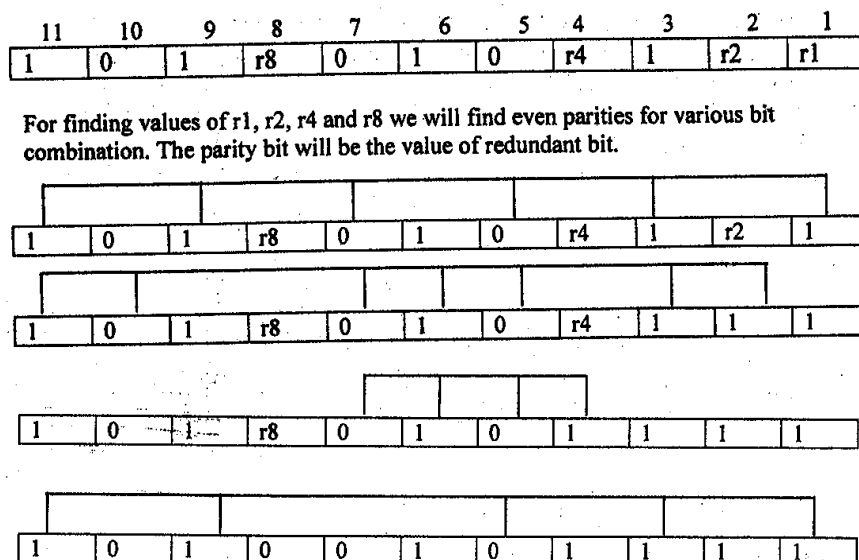
Figure 2.11: Forward Error Correction
