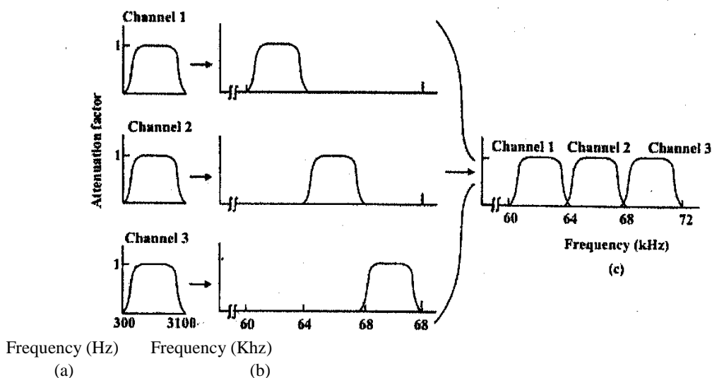
Figure 1.50: Frequency division multiplexing
