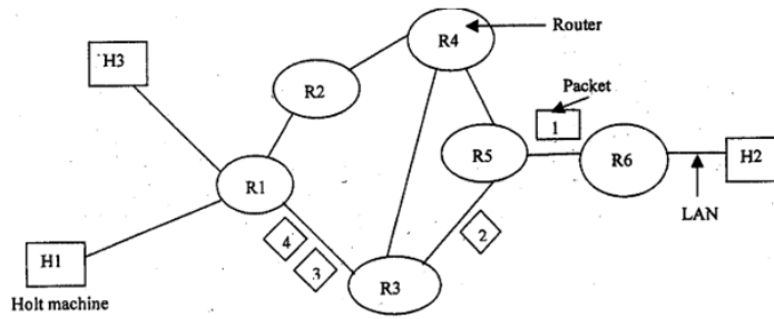
Figure 3.2: Routing in a virtual subnet
