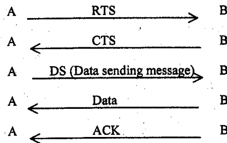
Figure 2.43: The MACAW protocol
