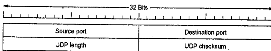
Figure 4.5: UDP segment structure
