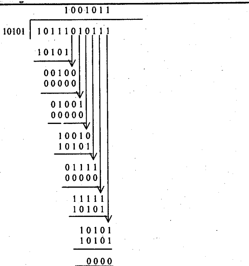
Figure 2.14: Cyclic redundancy check the receiver side
