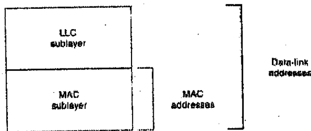
Figure 3.6: MAC addresses, data-link addresses, and the IEEE Sub-layer, of the data link layer are all related
