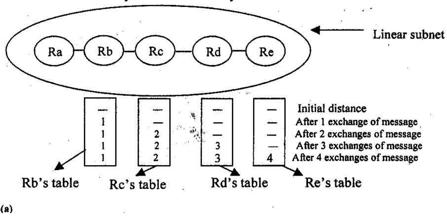
Figure 3.17(a): five node subnets
