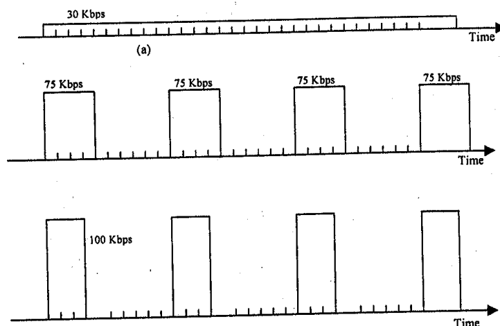
Figure 3.32: Possible traffic patterns at the average rate of 30 Kbps
