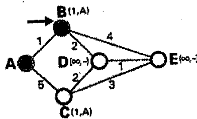
Figure 3.14(b) Dijkstra Algorithm b
