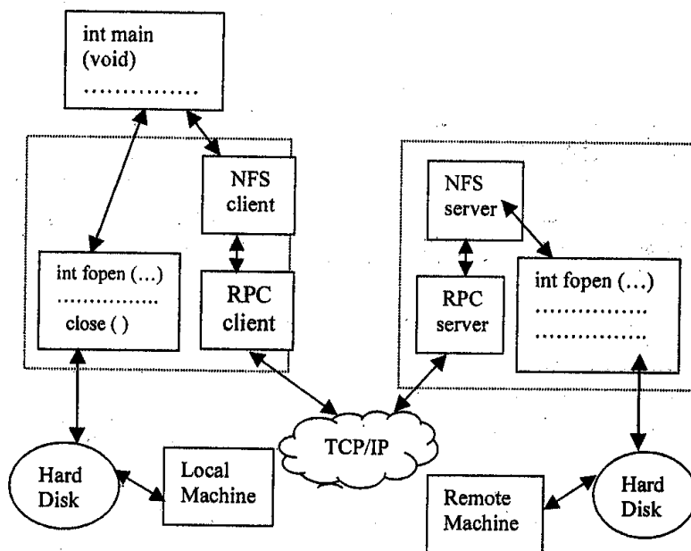
Figure 4.10: Concept of remote procedure call
