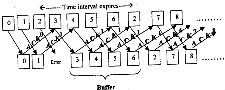
Figure 2.28: Pipelining in selective repeat
