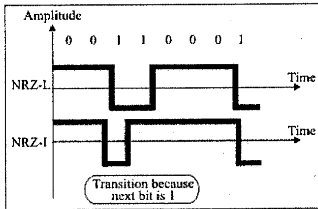
Figure 1.46: NRZ -L and NRZ-I encoding
