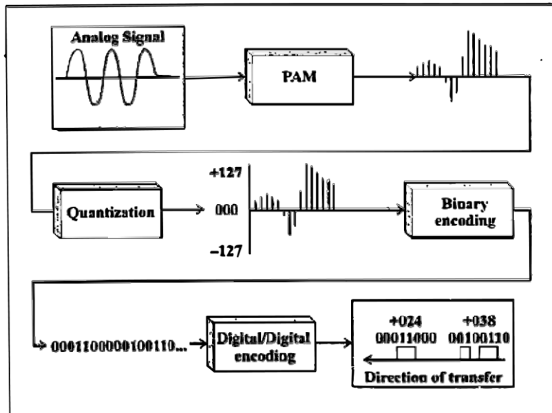
Figure 1.38 : Pulse Code Modulation
