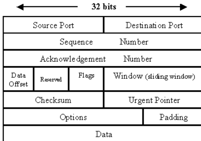
Figure 4.6: TCP header format
