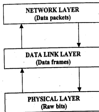
Figure 2.1: Data link layer providing services to network layer
