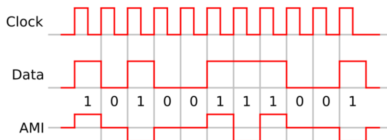
Figure 1.49: Bipola Encoding
