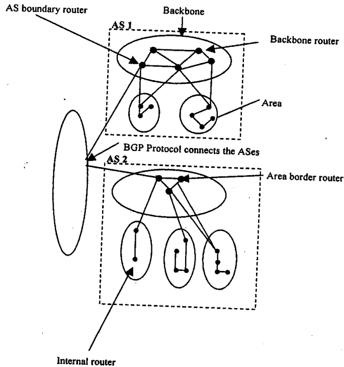
Figure 3.42: Working domain of OSPF
