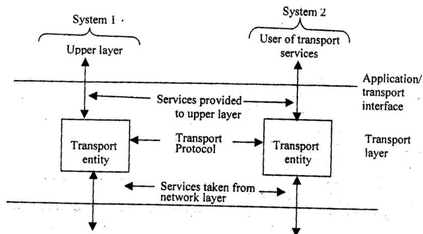
Figure 4.1: Transport entity environment
