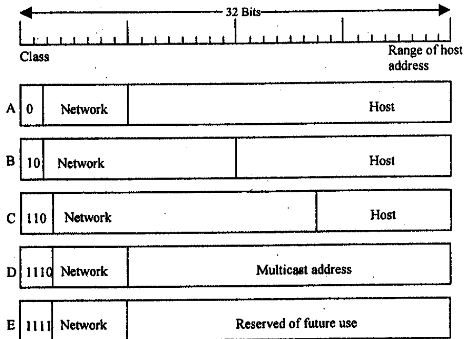
Figure 3.38 (b): IP address formats
