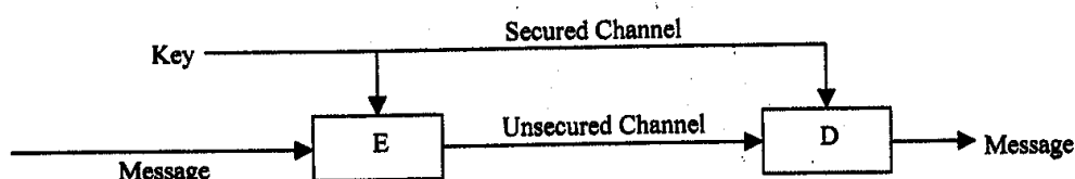
Figure 4.11: Secret Key Cryptography
