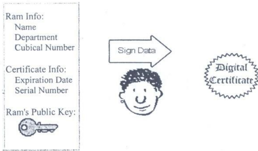
Figure 4.40: Creation of a digital certificate
