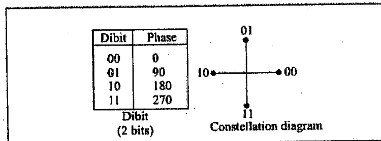
Figure 1.42: 4 PSK
