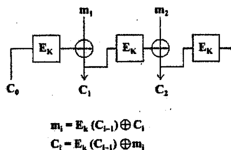
Figure 4.18: Cipher feedback model
