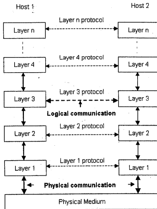
Figure 1.8: Layered network architecture
