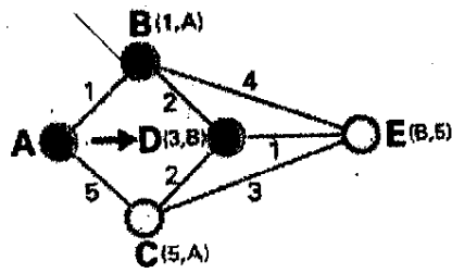
Figure 3.14 (c) Dijkstra Algorithm C
