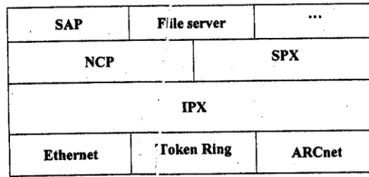
Figure 1.17: The Novell NetWare reference model
