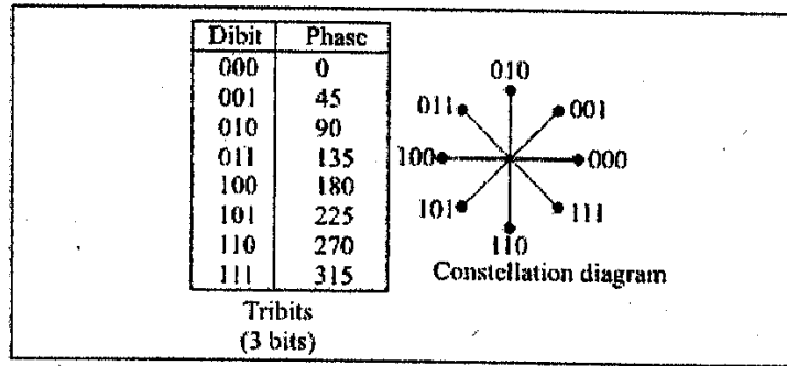
Figure 1.43: 8 PSK
