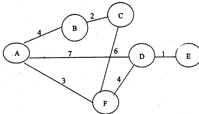
Figure 3.19: A subnet for link state routing
