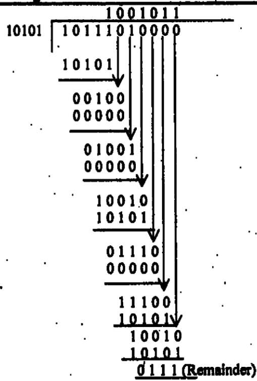
Figure 2.13: Cyclic redundancy check
