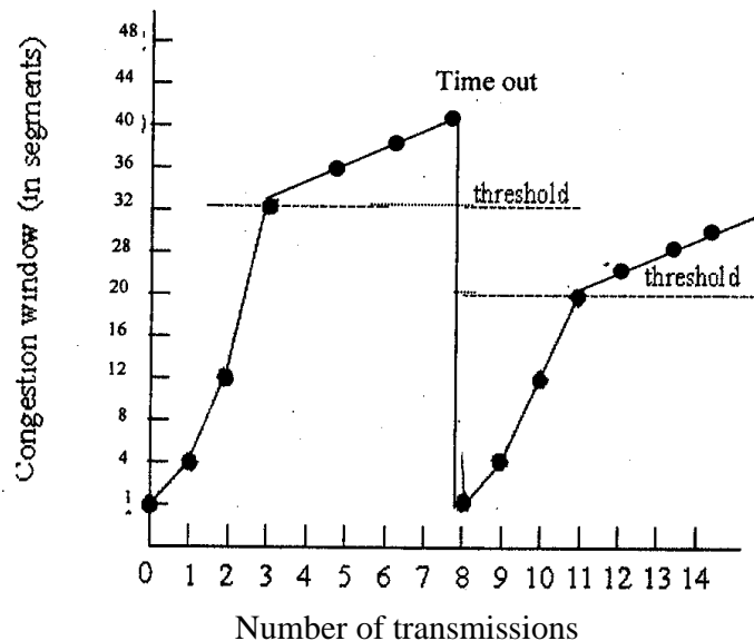
Figure 4.8: Dynamics of TCP congestion window
