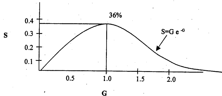
Figure 2.35: Throughput vs. load graph of slotted ALOHA
