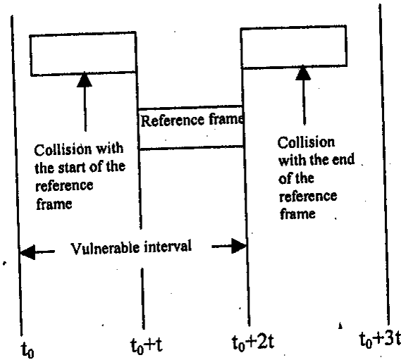
Figure 2.33: Vulnerable period
