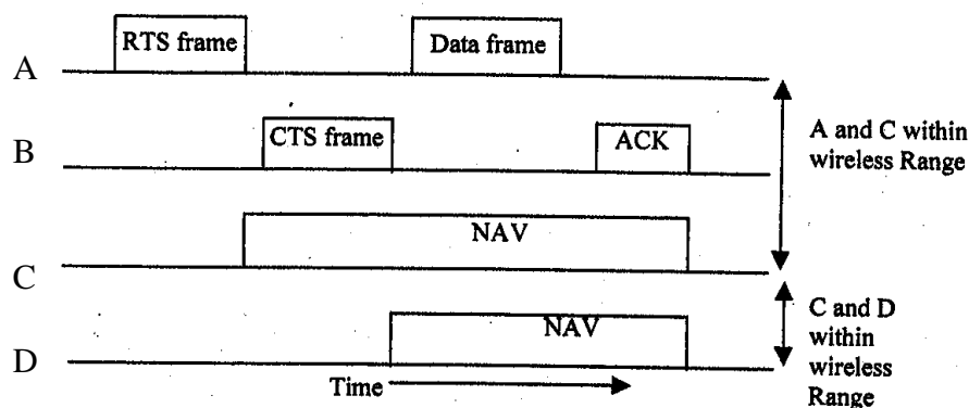
Figure 2.46: The use of virtual channel sensing using CSMA/CA
