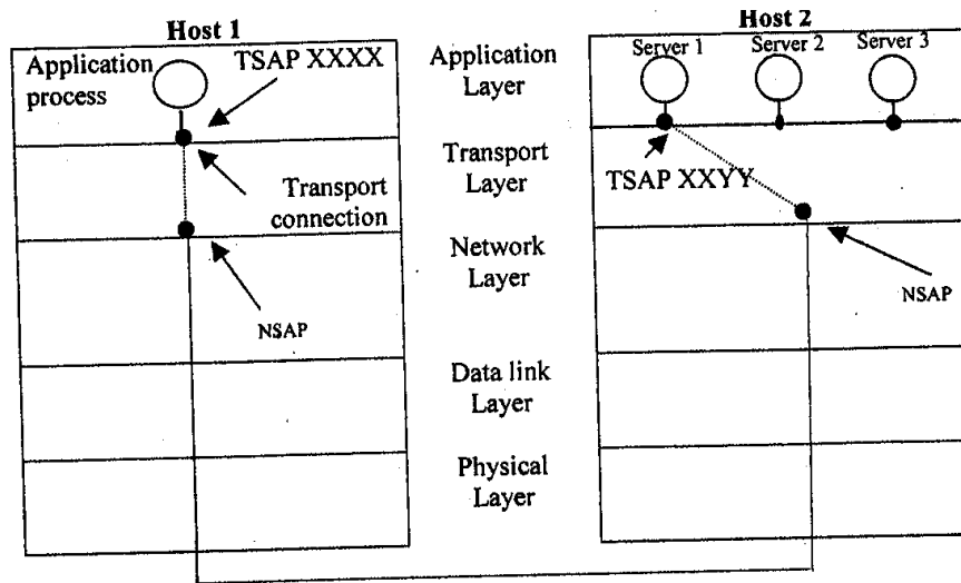
Figure 4.2: Transport connections between a client and a server
