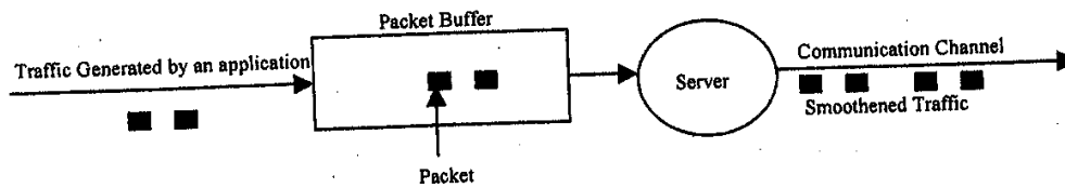
Figure 3.33: A leaky bucket traffic shaper
