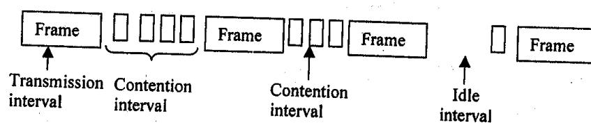
Figure 2.37: Transmission states
