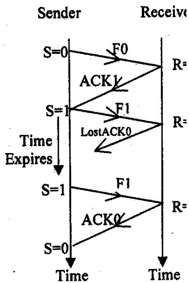
Figure 2.21: Loss of ACK
