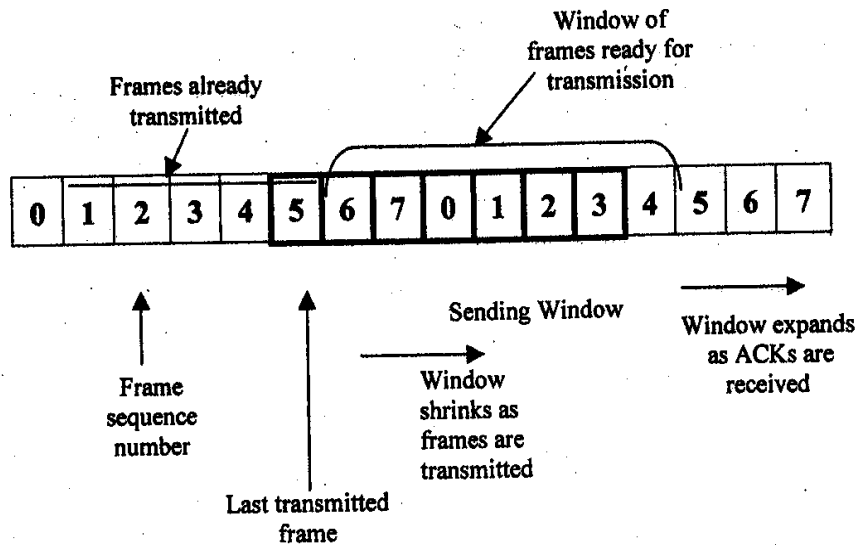
Figure 2.17: Sending Window in I Sliding Window
