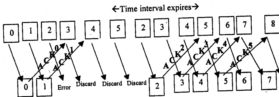
Figure 2.27: Pipelining in Go-Bank-N
