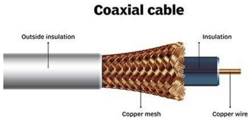
Figure 1.30 : Coaxial cable
