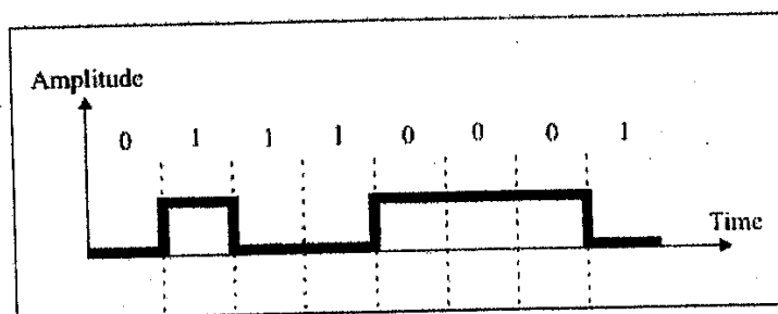
Figure 1.45: Unipolar encoding
