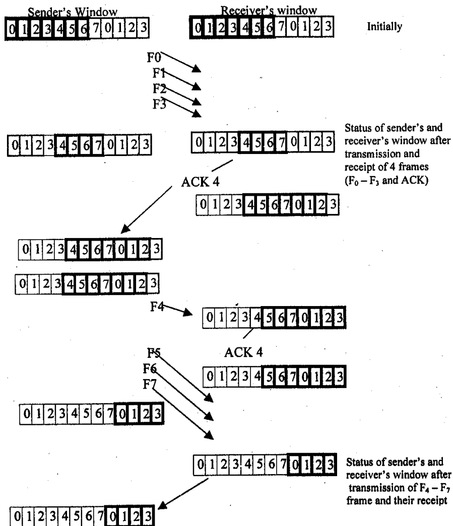
Figure 2.19: Function of a sliding window machine
