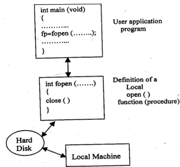
Figure 4.9: Concept of local procedure call
