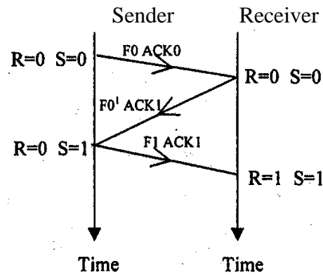
Figure 2.29: Piggybacking
