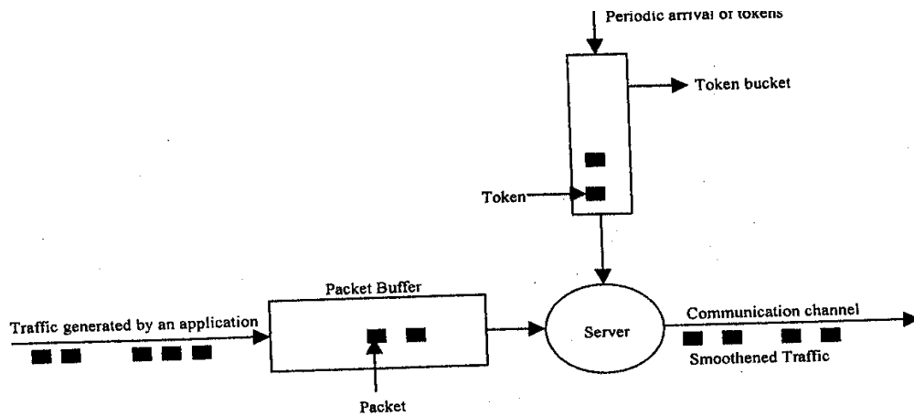
Figure 3.34: Token bucket traffic shaper
