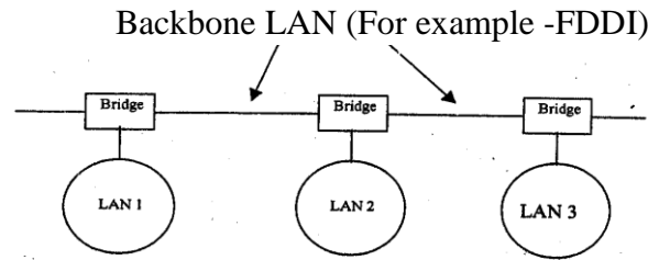
Figure 2.48: Multiple LANs connected by backbone to handle a total load higher than the capacity of single LAN
