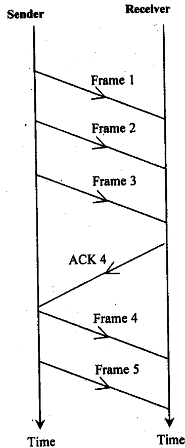
Figure 2.16: Normal flow diagram of sliding
