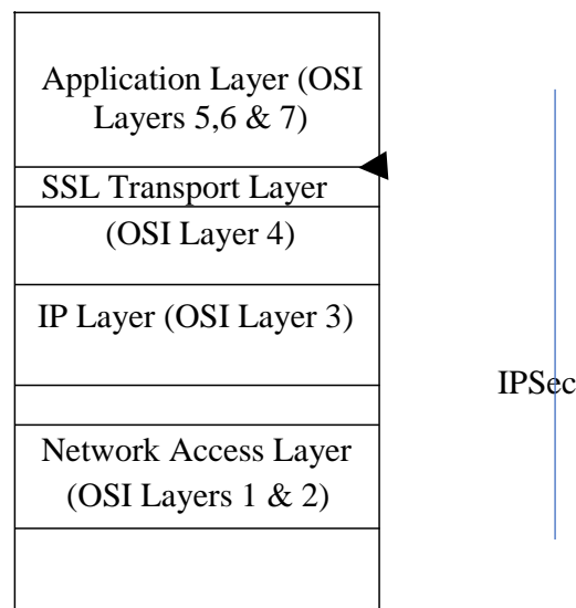
Figure 4.49: Protocol redirector
