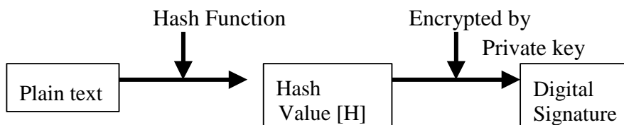
Figure 4.31: Digital signature
