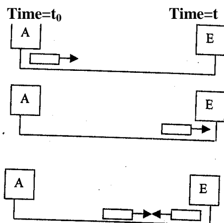
Figure 2.36: Collision detection
