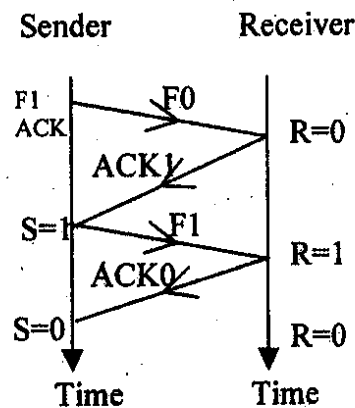
Figure 2.20: Stop and wait protocol
