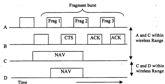
Figure 2.47: A fragment burst
