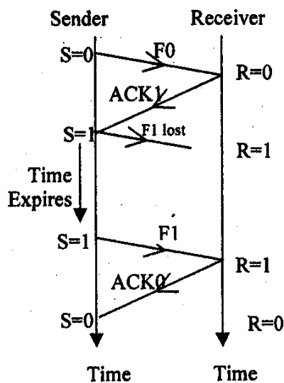
Figure 2.22: Loss of a frame
