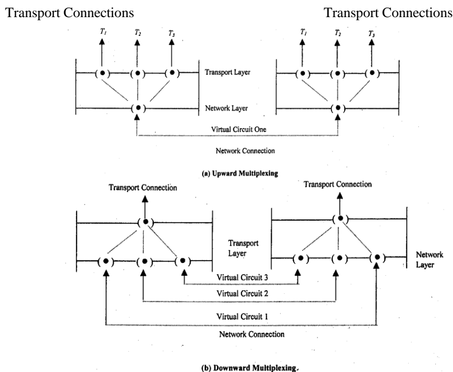
Figure 4.3: Multiplexing
