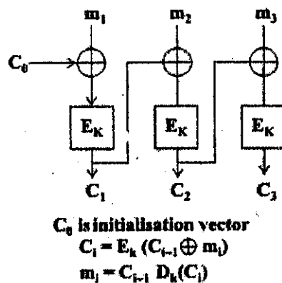
Figure 4.17: Cipher block chaining
