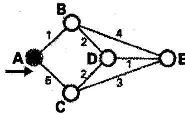
Figure 3.14(a) Dijkstra Algorithm A
