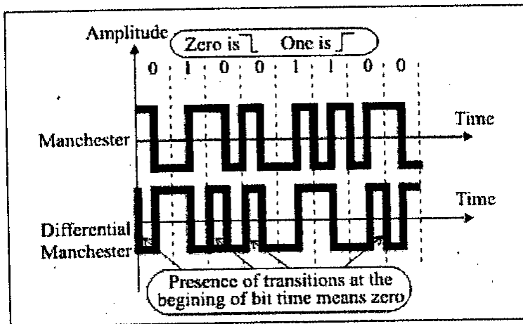
Figure 1.48: Manchester and differential Manchester encoding
