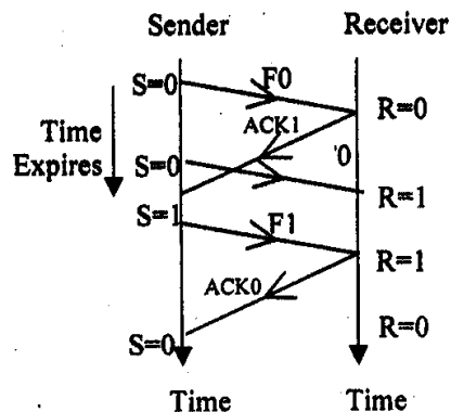
Figure 2. 23: ACK lime out
