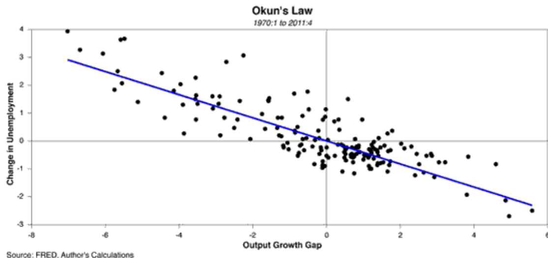
Figure 1: Okun's Law
