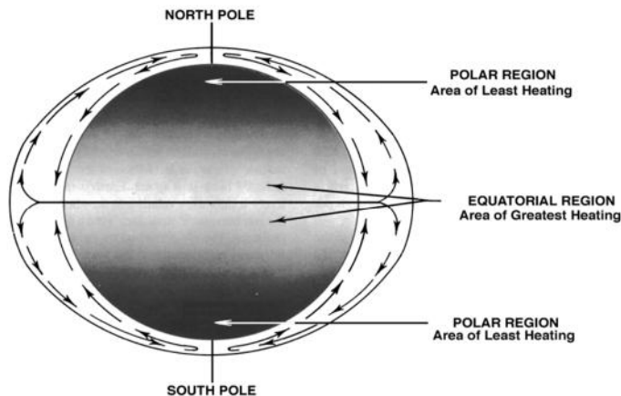
Fig. 3.1: Ideal Atmospheric Circulation for a Uniform and Non-Rotating Earth
