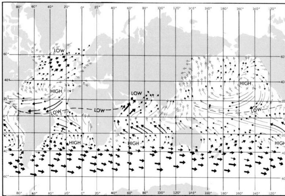
Fig. 3.4: Generalised Pattern of Actual Surface Winds in July and August (See key with Figure 3.3)
