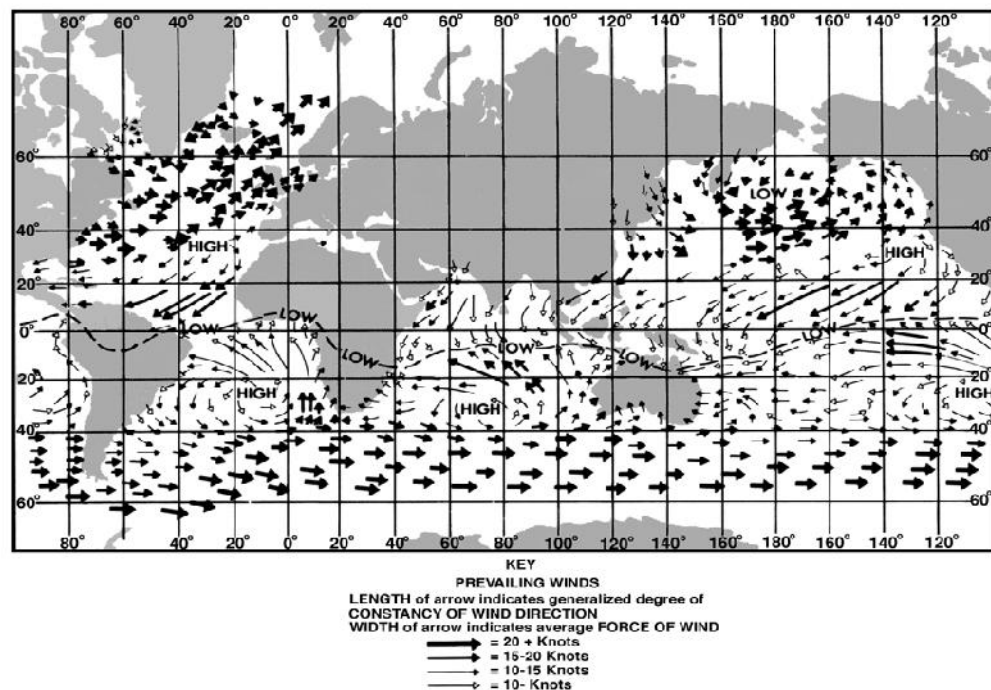
Fig. 3.3: Generalised Pattern of Actual Surface Winds in January and February
