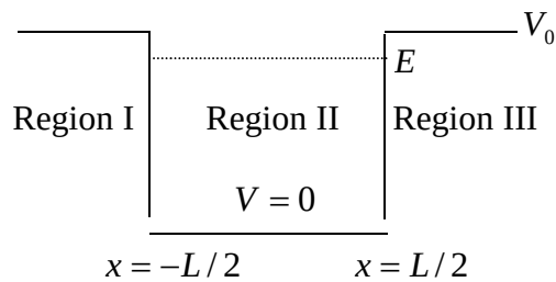
Fig. 1.3: The finite potential well of depth V_0 and width L . When E < V_0 , a particle in the potential is said to be bound. Compared to the infinite potential well, it is more convenient to take the centre of the well as x = 0 .
