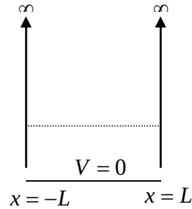
Fig. 3.1: The infinite square well potential confining a particle to a region of width L
