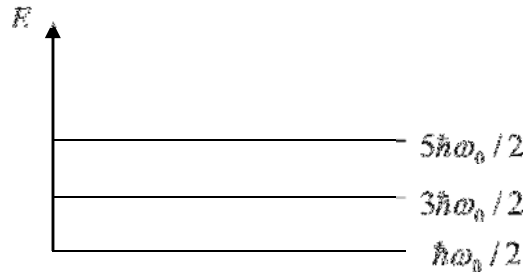
Fig. 1.1: The energy levels of the quantum-mechanical harmonic oscillator
