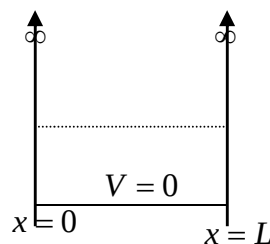
Fig. 1.1: The infinite square well potential confining a particle to a region of width L
