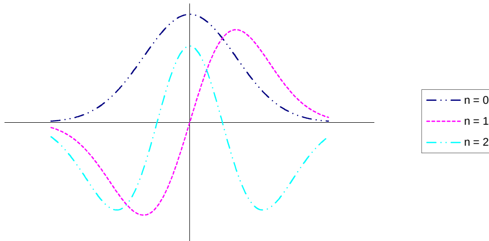
Fig. 1.2: Eigenfunctions of the quantum-mechanical harmonic oscillator
