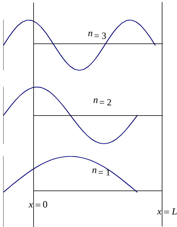
Fig. 1.2: The lowest three wavefunctions (for n = 1, 2 and 3 ) in the infinite square well potential.
